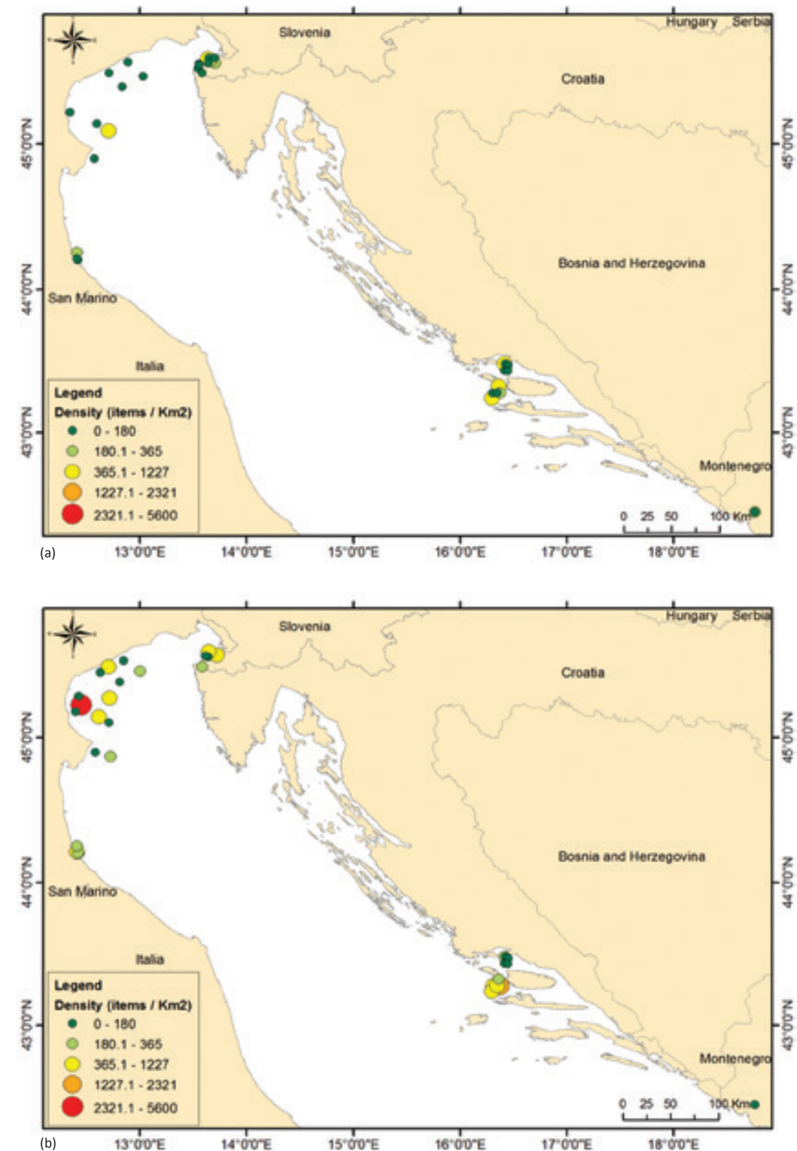
Figure 3.5. Spatial distribution of floating litter densities for the 66 transects conducted in coastal Adriatic waters: (a) in autumn 2014; and (b) in spring 2015.
