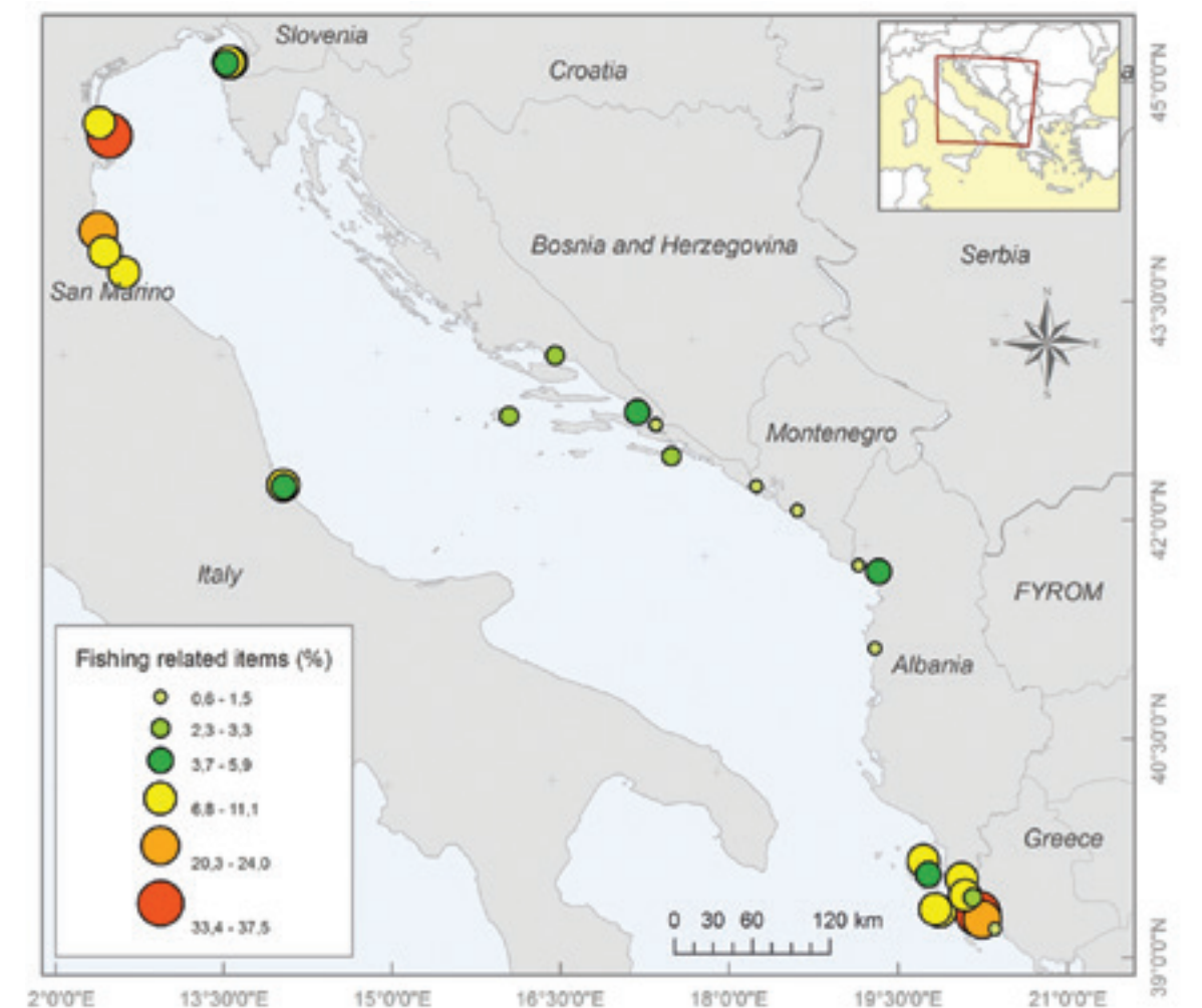
Figure 2.22. Spatial distribution of the amount of fishing related items (%) for the 31 survey sites located on coasts of the Adriatic and Ionian Seas.
